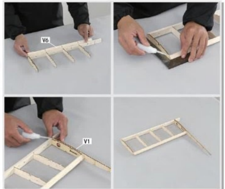
3.2 Glue V1 and V6 in place. Make sure plywood side of V1 is facing V2.
