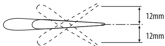
Aileron Control
